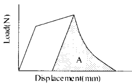
Figure 5. Load-Displacement curve.
