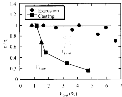
Figure 6. Dependence of \tau / \tau_i on V_{f,eff} .
