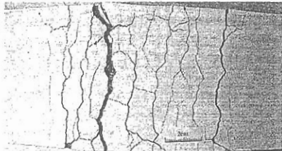
Fig. 9 - Ultimate State of Specimen Series 6 (2 Layers of Mesh ES1, with PVA fiber V_f=2.0\% )
