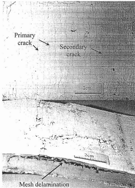
Fig. 11—Ultimate State of the Hybrid Composite with Kevlar Mesh and Spectra Fiber (Mesh is in Longitudinal Direction.)
