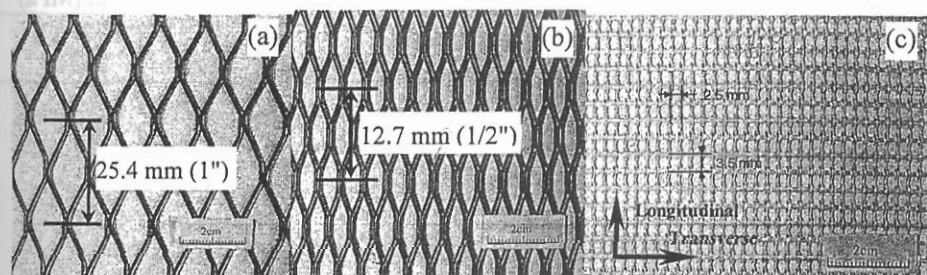
Fig. 1— (a) Expanded Steel Mesh ES1 with 25.4mm (1") Opening (b) Expanded Steel Mesh ES2 with 12.7mm (1/2") Opening (c) Kevlar Mesh, 1500 Denier per Yarn
