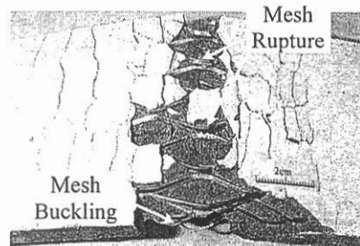
Fig. 4 — Ultimate State of Specimen Series 2 (2 Layers of Mesh ES1, w/o fiber)
