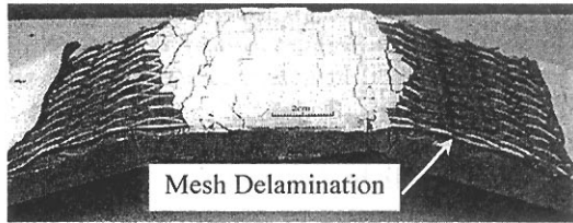
Fig. 5 – Ultimate State of Specimen Series 3 (2 Layers of Mesh ES2, w/o fiber)
