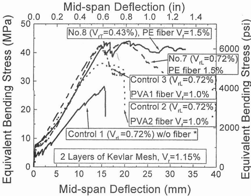
Fig. 10 – Average Stress-Deflection Curves of Hybrid Ferrocement with 2 Layers of Kevlar Mesh and Discontinuous Fibers (* see ref [13])
