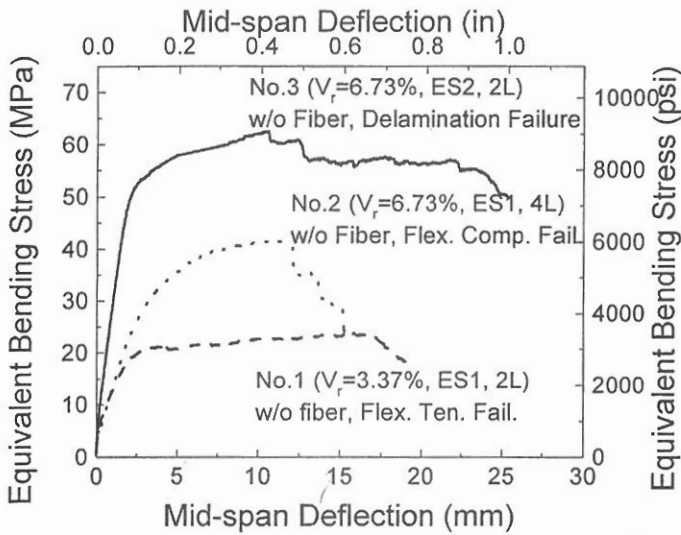
Fig. 2—Average Stress-Deflection Curves of Series 1 to 3
