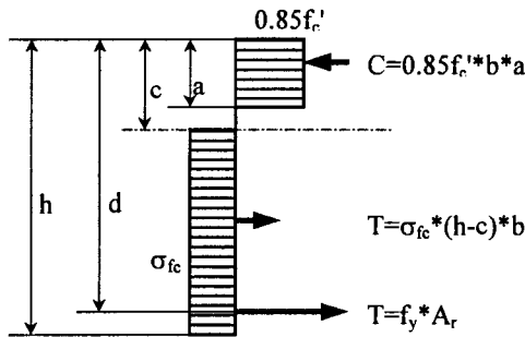
Fig. 13– Stress Distribution at the Cross-Section of Hybrid Composite with Steel Mesh and Fiber
