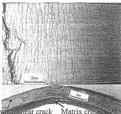
Fig.8- Ultimate State of Specimen Series 5 (2 Layers of ES2, with Spectra fiber V_f=1.5\% )
