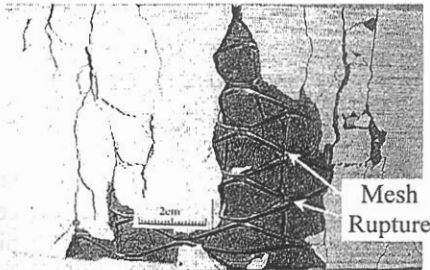
Fig. 3 — Ultimate State of Specimen Series 1 (4 Layers of Mesh ES1, w/o fiber)
