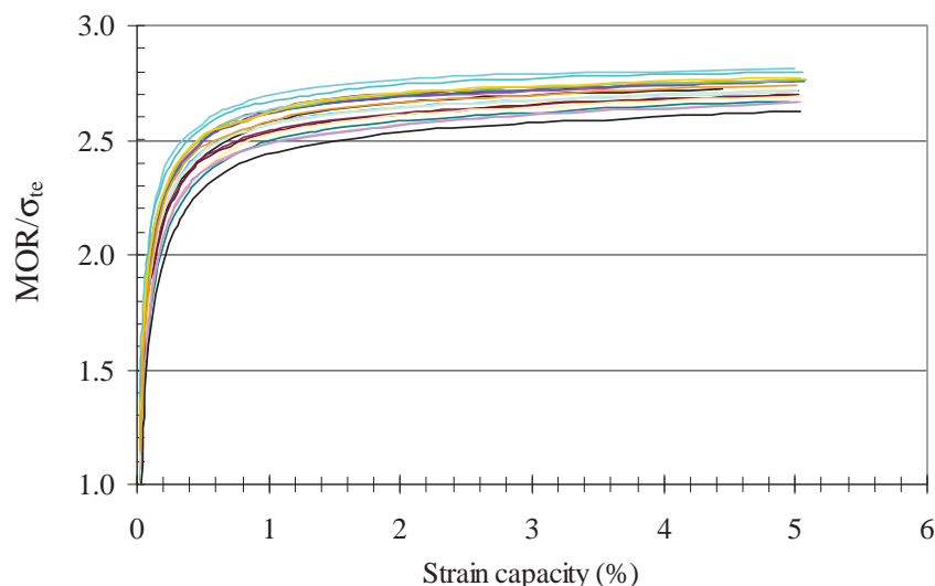
Figure 2: Relation of MOR/\sigma_{te} with strain capacity for all cases with UM/JCI data
