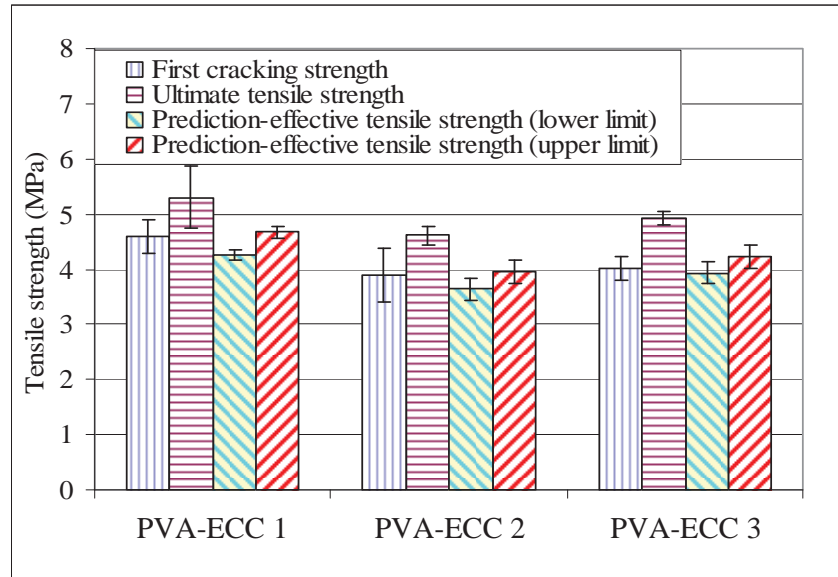
Figure 4: Comparison of UTT results and predicted effective tensile strength based on extended UM method for PVA-ECC 1, 2 and 3
