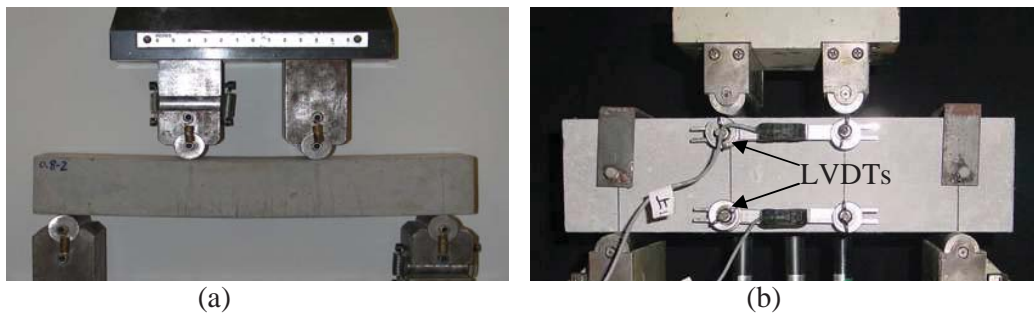
Figure 3: Comparison of test setup for the (a) UM method and (b) JCI method (Beam deflection at the loading points was obtained from machine displacement directly in UM method)
